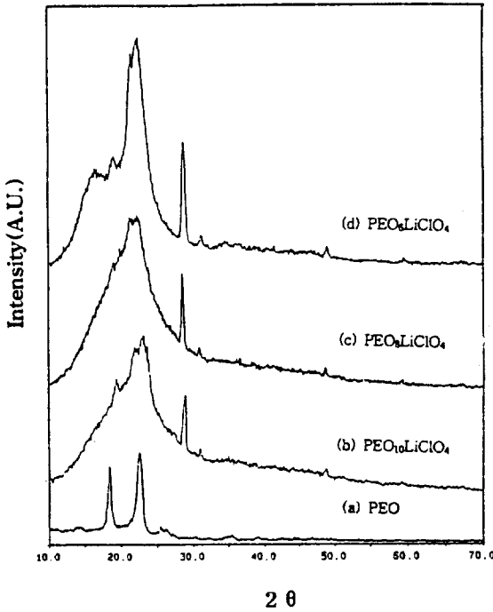
그림 5. \text{PEO}_x\text{LiClO}_4 전해질 필름의 X-선 회절 패턴. Fig. 5. X-ray diffraction patterns of \text{PEO}_x\text{LiClO}_4 electrolyte film as a function of Li salt concentration.
