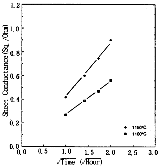
Fig. 4 Sheet conductance versus square root of diffusion time at 1100 and 1150°C.
