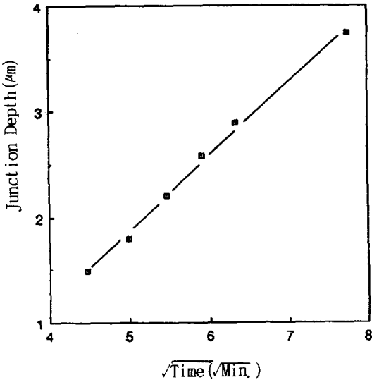
Fig. 7 Junction depth versus square root of time for doping at 1150°C
