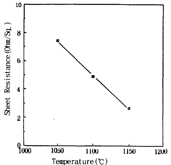
Fig. 3 Variation in sheet resistance with diffusion temperature for 1 hour doping.
