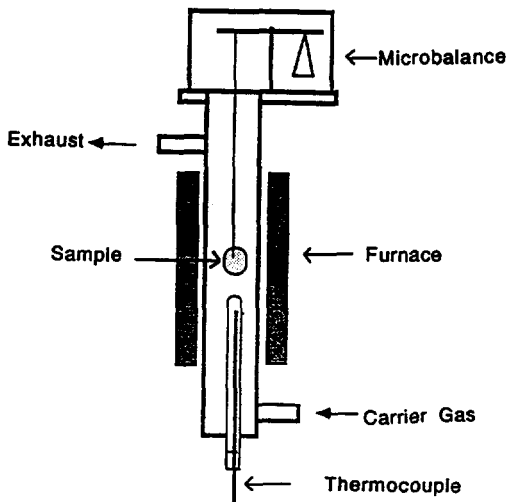
Fig. 1. Schematic diagram of the thermogravimetric analysis system.
