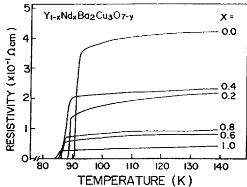
Fig. 3. Electrical resistivity versus temperature as a function of Nd content X in Y_{1-x}Nd_xBa_2Cu_3O_{7-y} samples
