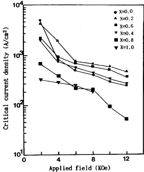
Fig.8. Field dependence of the critical current densities at 30K for Y_{1-x}Nd_xBa_2Cu_3O_{7-y}
