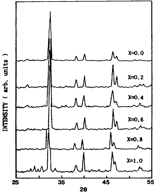
Fig. 1. X-ray diffraction patterns of Y_{1-x}Nd_xBa_2Cu_3O_{7-y}
