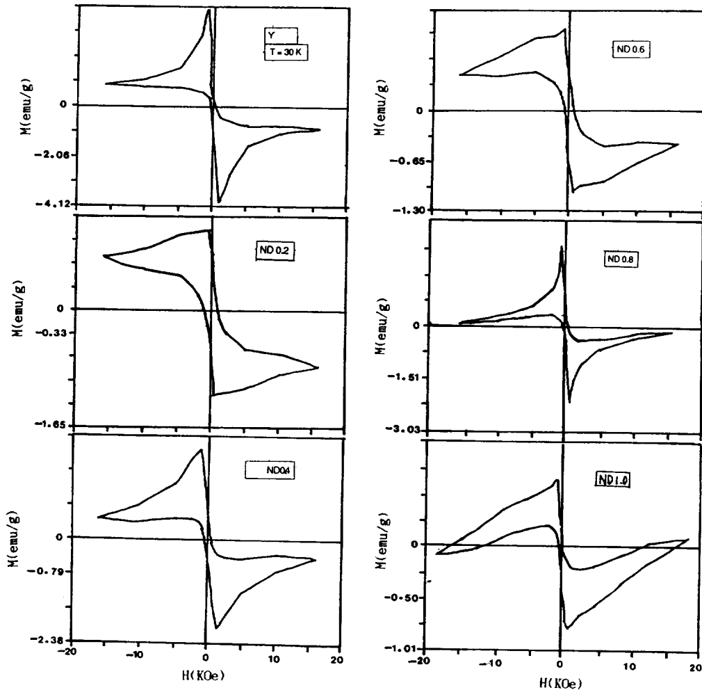
Fig.6. Magnetic hysteresis curves at 30K up to the maximum external field of 16KOe for Y_{1-x}Nd_xBa_2Cu_3O_{7-y} .
