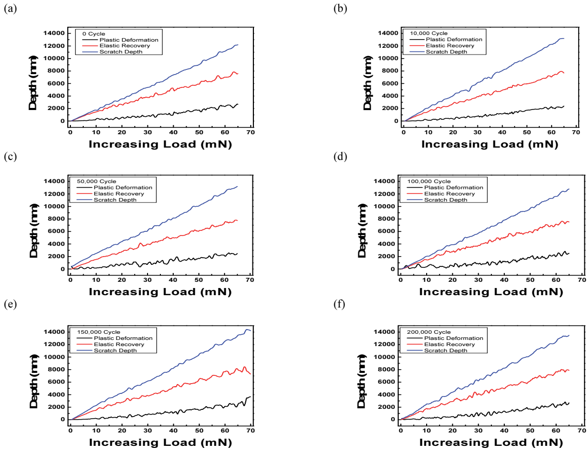
Fig. 6. Vertical scratch test. (a) 0 cycle, (b) 10,000 cycles, (c) 50,000 cycles, (d) 100,000 cycles, (e) 150,000 cycles, and (f) 200,000 cycles.
