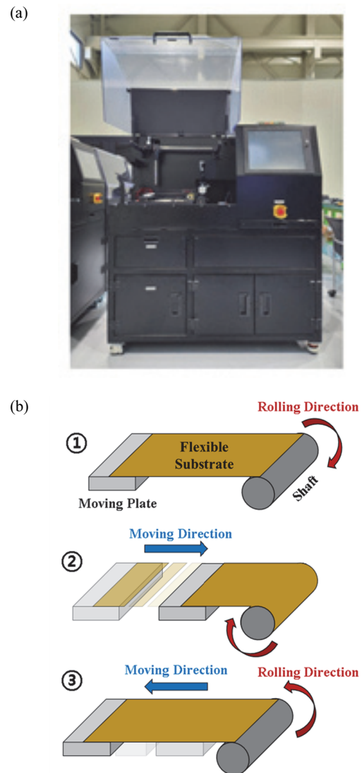
Fig. 1. Rolling test. (a) Rolling equipment and (b) rolling mechanism.
