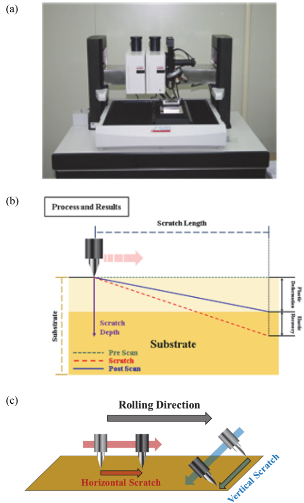
Fig. 3. Scratch test. (a) Scratch equipment, (b) scratch test mechanism, and (c) scratch direction.
