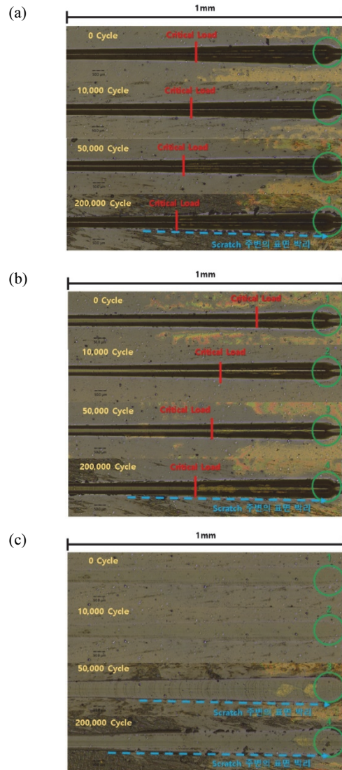
Fig. 8. Microscopic observation of PI film surface according to indenter size. (a) 10 \mu\text{m} , (b) 20 \mu\text{m} , and (c) 100 \mu\text{m} .
