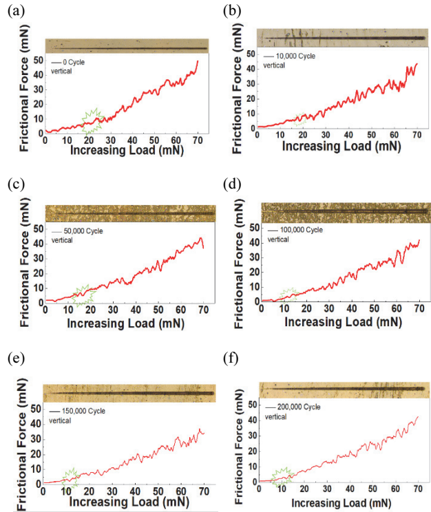
Fig. 4. Vertical critical load according to rolling cycles. (a) 0 cycle, (b) 10,000 cycles, (c) 50,000 cycles, (d) 100,000 cycles, (e) 150,000 cycles, and (f) 200,000 cycles.
