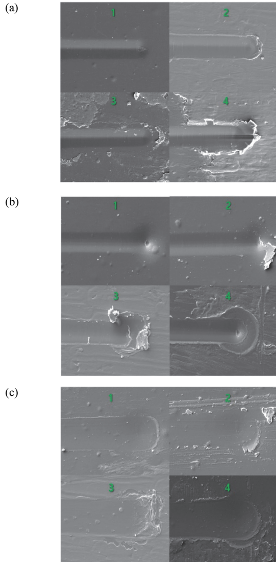
Fig. 9. SEM images of PI film surface as a function of indenter size (a) 10 \mu\text{m} , (b) 20 \mu\text{m} , and (c) 100 \mu\text{m} .
