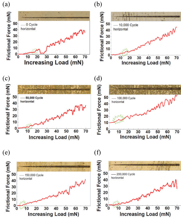
Fig. 5. Horizontal critical load according to rolling cycles. (a) 0 cycle, (b) 10,000 cycles, (c) 50,000 cycles, (d) 100,000 cycles, (e) 150,000 cycles, and (f) 200,000 cycles.
