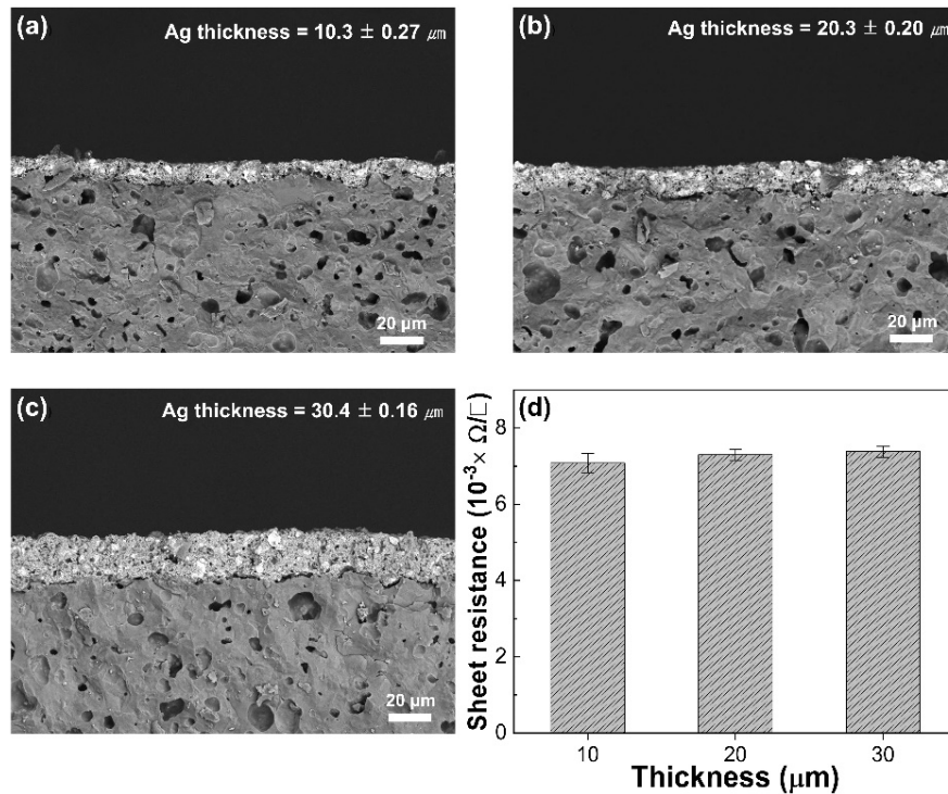
Fig. 3. Cross-sectional SEM image of the Ag layer on the ceramic container according to the number of deposition processes through the screen-printing method: (a) 1 time, (b) 2 times, and (c) 3 times.
