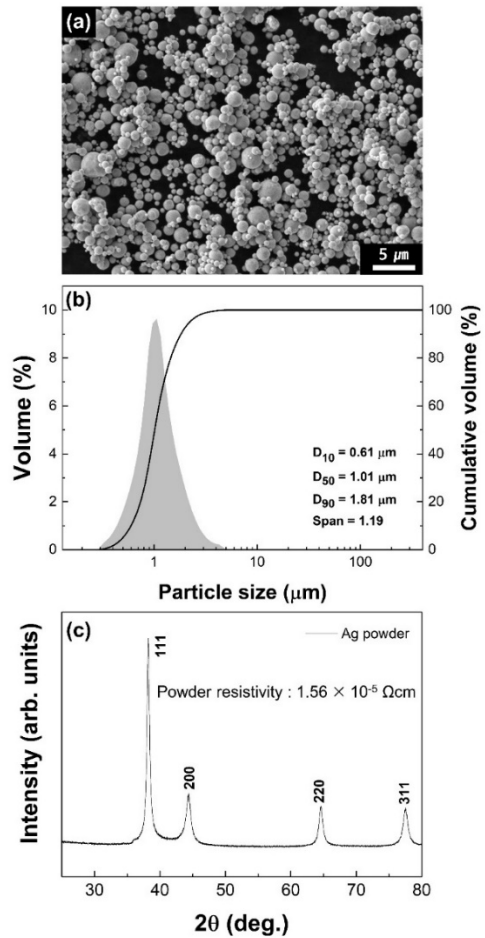
Fig. 2. (a) SEM image, (b) particle size distribution, and (c) XRD pattern of Ag powder.
