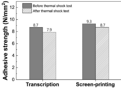
Fig. 6. Strain of adhesion strength after thermal shock test according to each process.
