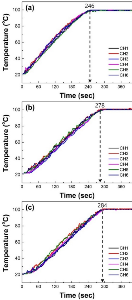
Fig. 4. Results of the time to raise 1 L of the water to 100°C at R.T. (a) Ag metal pot, (b) transcription method, and (c) screen-printing method.
