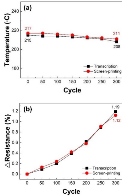
Fig. 5. (a) Temperature deviation and (b) the rate of changes in resistance of ceramic plate with Ag layer by transcription and screen-printing according to temperature cycle test.
