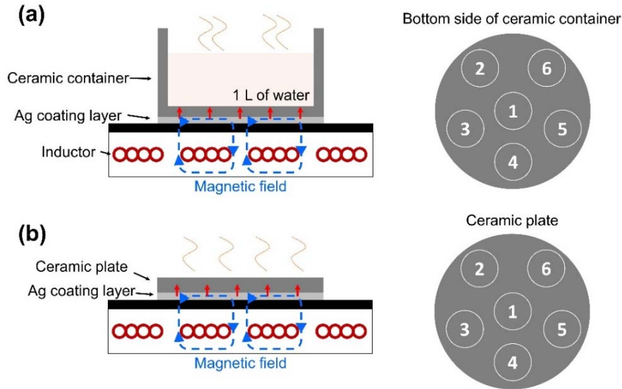
Fig. 1. Schematic diagram of (a) thermal conductivity performance of ceramic container with Ag coating layer and (b) reliability evaluation through temperature cycle test of heat cycle test of ceramic plate coated with Ag film.
