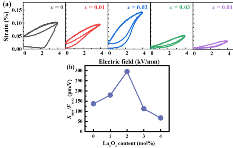
Fig. 5. (a) Unipolar strain curves and (b) variation of S_{max}/E_{max} for BNLST100xLa ceramics as a function of La_2O_3 content.
