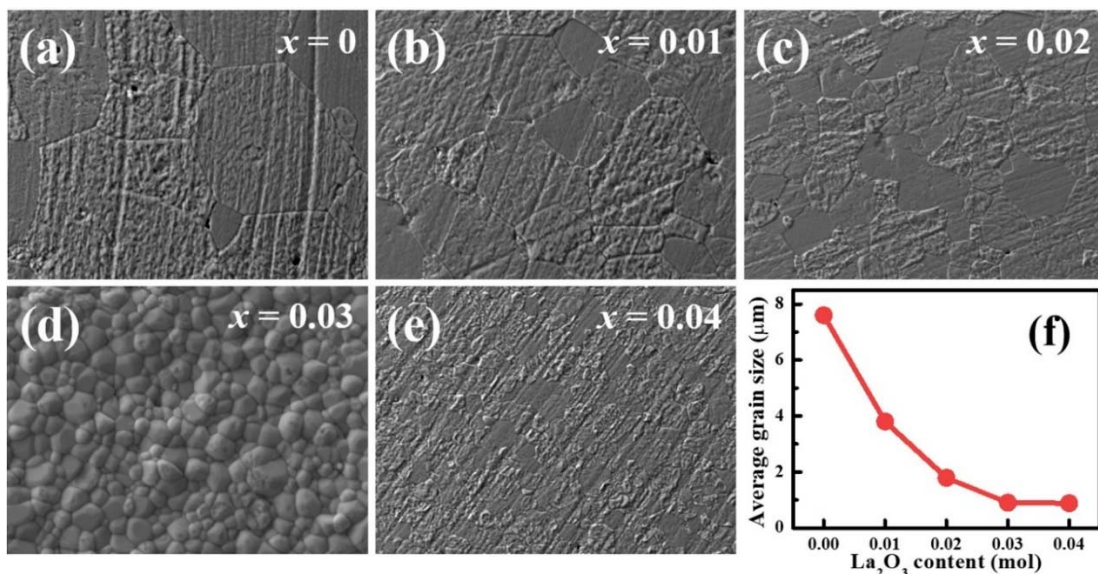
Fig. 1. Polished and thermally etched surface images of BNLST100xLa ceramics, (a) x = 0 , (b) x = 0.01 , (c) x = 0.02 , (d) x = 0.03 , (e) x = 0.04 , and (f) average grain size as a function of \text{La}_2\text{O}_3 content.
