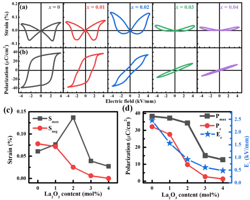
Fig. 4. Electric field induced (a) bipolar strain ( S - E ) curves, (b) polarization ( P - E ) hysteresis, the extracted, (c) S_{\text{max}} and S_{\text{neg}} , and (d) P_{\text{max}} , P_r , and E_c values for BNLST100xLa ceramics as a function of La 2 O 3 content.
