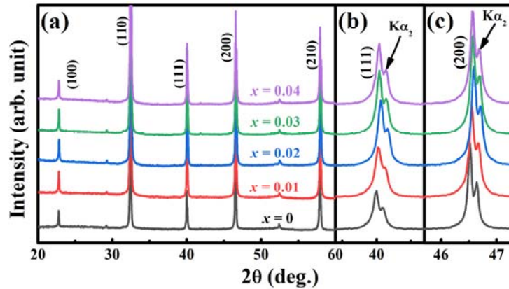
Fig. 2. X-ray diffraction patterns of BNLST100xLa ceramics as a function of \text{La}_2\text{O}_3 content, 2\theta range of (a) 20\sim 60^\circ , (b) 39.4\sim 40.7^\circ , and (c) 45.7\sim 47.3^\circ .
