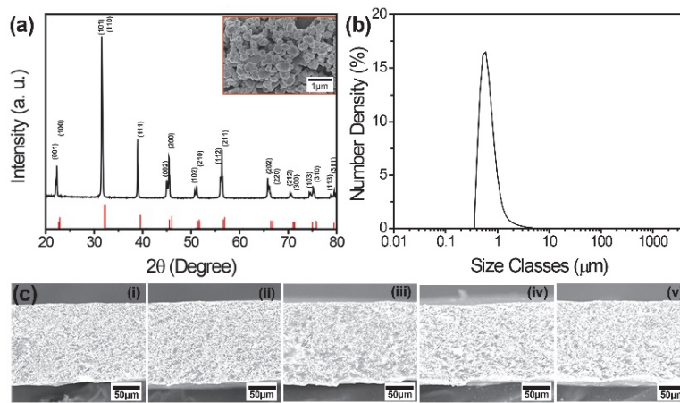
Fig. 2. (a) XRD pattern and SEM image (insert) of the synthesized piezoelectric BaTiO 3 nanoparticles, (b) particle size analysis results of BaTiO 3 nanoparticles, and (c) cross-sectional SEM image of the piezoelectric composite layer with various BaTiO 3 -CNTs concentrations.
