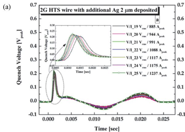
Fig. 7. Quench voltage of 2G HTS wire additional deposition (a) Ag 2 \mu m and (b) Ag 3 \mu m .
