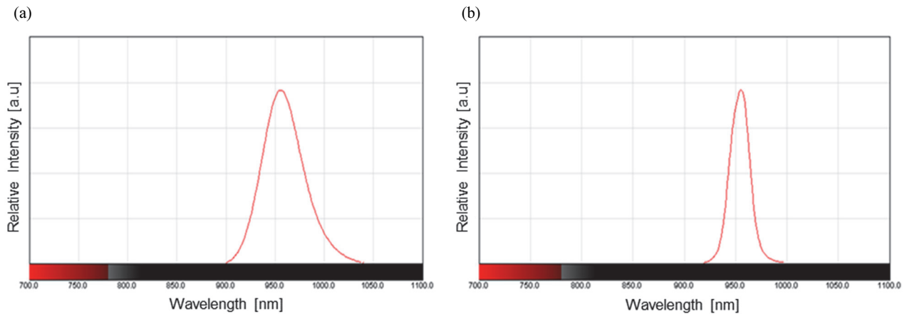
Fig. 9. Radiant intensity of 945 nm NIR LED without and with e-beam deposited \text{SiO}_2/\text{TiO}_2 multi-layers narrow band pass filter. (a) No filter and (b) with filter.
