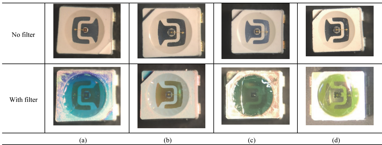
Fig. 5. The USB microscope images for surfaces of IR and NIR LEDs without and with SiO 2 /TiO 2 multilayers narrow band pass filter. (a) 640 nm, (b) 830 nm, (c) 880 nm, and (d) 956 nm.
