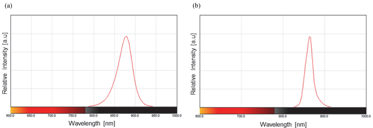
Fig. 8. Radiant intensity of 880 nm NIR LED without and with e-beam deposited \text{SiO}_2/\text{TiO}_2 multi-layers narrow band pass filter. (a) No filter and (b) with filter.
