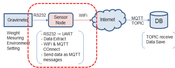
Fig. 2. Data transmission configuration diagram.
