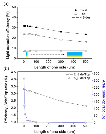
Fig. 6. (a) Result of light extraction efficiency and (b) side/top ratio according to changing the length of one side of the non PSS FC \mu -LEDs.
