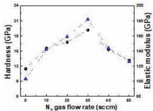
Fig. 4. Hardness and elastic modulus values in TiN thin films fabricated with the increase of N 2 gas flow rate.
