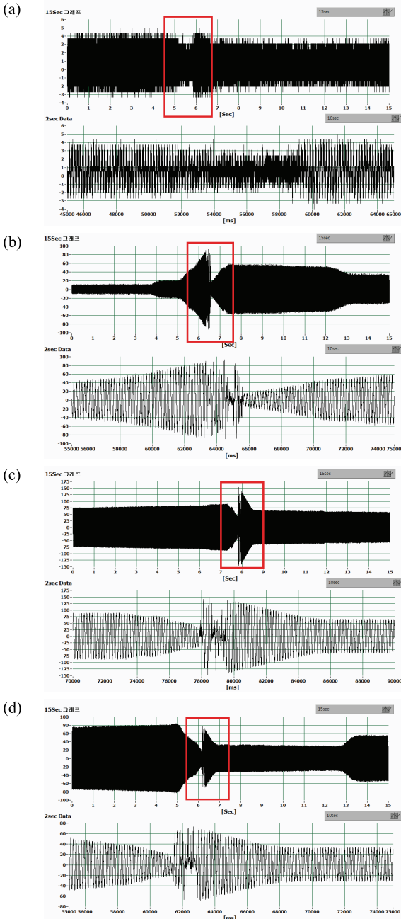
Fig. 3. Results of current wave from between contact and catenary wire of HEMU-430X on Honam HSR, (a) 159 km/h, (b) 290 km/h, (c) 349 km/h, and (d) 370 km/h.
