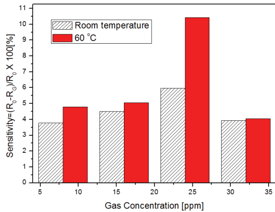
Fig. 5. Sensitivity of MWCNT/ZnO composite film gas sensor.
