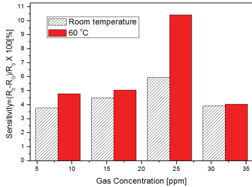
Fig. 5. Sensitivity of MWCNT/ZnO composite film gas sensor (diagonal line is room temperature, red line is chamber temperature at 60°C).
