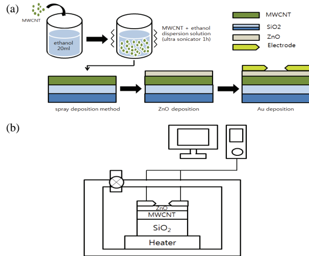
Fig. 1. (a) Schematic structure of the processes in the fabrication of the NO x gas sensor, and (b) gas sensor measurement system using the Elvis device.
