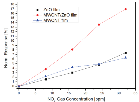
Fig. 4. Normalized response of gas sensor by NO x gas detections.
