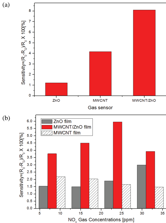
Fig. 3. (a) Sensitivity of gas sensor for NO x gas 16 ppm as the ZnO, MWCNT film and MWCNT/ZnO film and (b) analysis of comparison from the variation of NO x gas concentrations.
