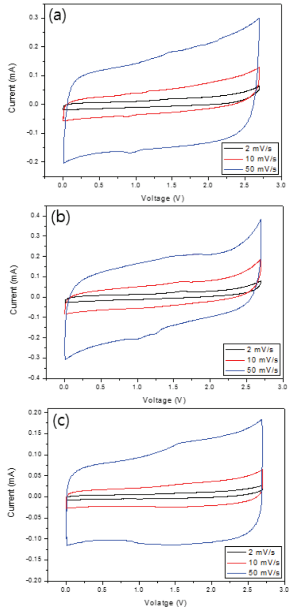
Fig. 4. Cyclic voltammograms of (a) G-3nm, (b) G-12nm, and (c) G-60nm at 2, 10, 50 mV/s scan rates.
