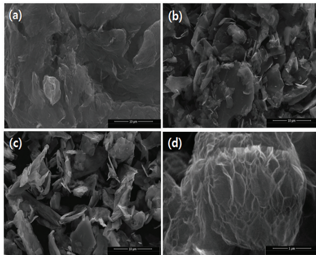
Fig. 1. SEM image; (x10,000) (a) G-3nm, (b) G-12nm, (c) G-60nm, and (x100,000) (d) G-3nm.
