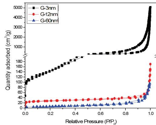
Fig. 2. Nitrogen-adsorption isotherm at 77 K for graphene flakes with diverse sizes.
