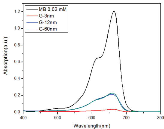
Fig. 3. Metylen blue adsorption for electrodes with diverse sizes of graphene flakes.
