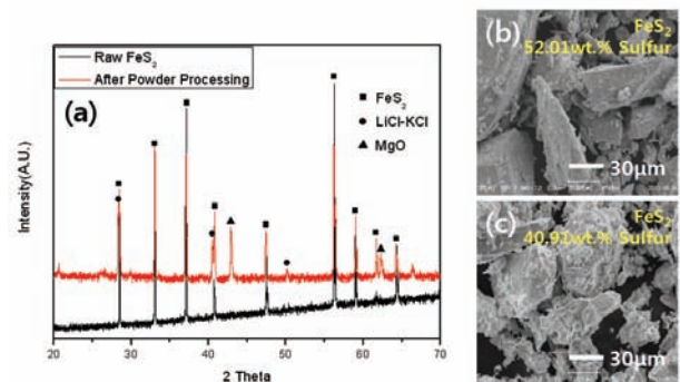
Fig. 1. (a) XRD and (b-c) SEM results of raw FeS_2 and powder processed cathode powders.
