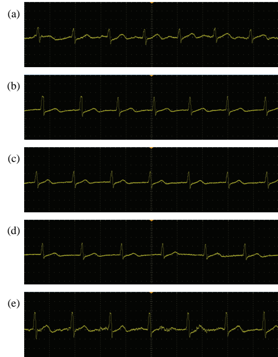
Fig. 9. ECG signals of real human according to different electrode diameters. (a) 10, (b) 40, (c) 50, (d) 60, and (e) 70 mm.
