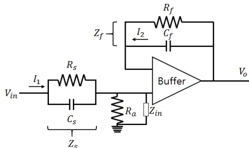
Fig. 4. Proposed buffer circuit for impedance matching.
