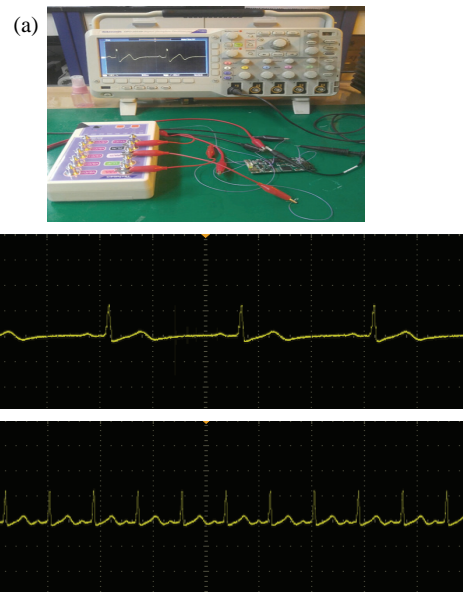
Fig. 6. (a) ECG measurement system, (b) 35 bpm ECG signal, and (c) 130 bpm ECG signal generated by ECG simulator.
