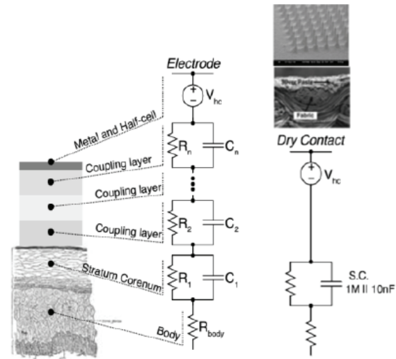
Fig. 2. Equivalent circuit of skin-electrode interface.
