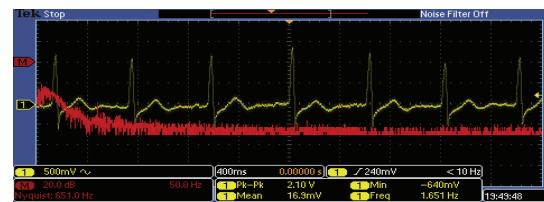
Fig. 7. ECG signal spectrum of real human at 0.05-100 Hz band.
