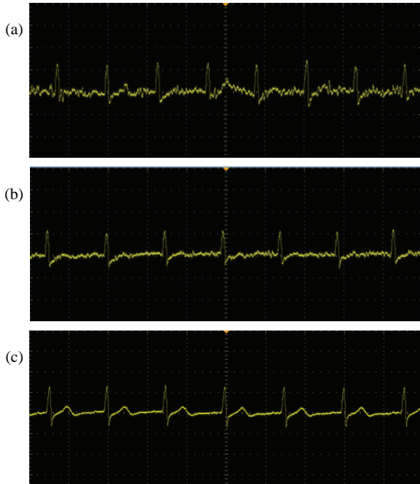
Fig. 8. ECG signals of (a) Fig. 5(a) electrode, (b) Fig. 5(b) electrode, and (c) Fig. 5(c) electrode.
