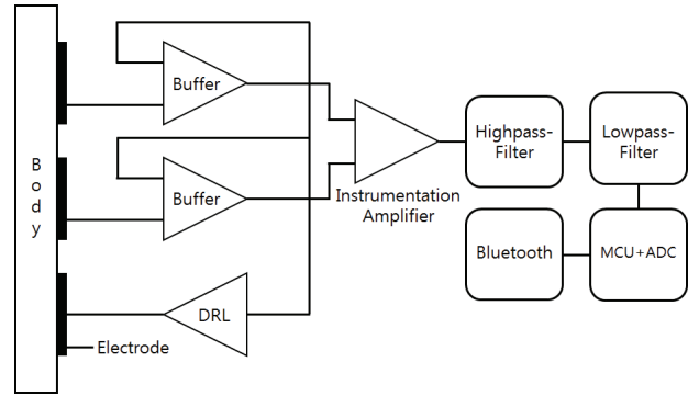
Fig. 1. Block diagram of ECG circuit.
