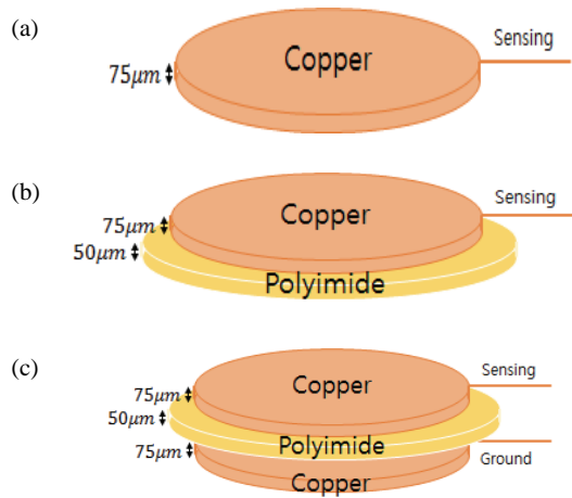
Fig. 5. Structures of proposed electrode.
