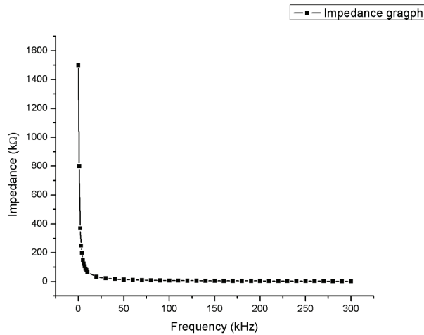
Fig. 3. Impedance measurement between skin and electrode according to frequency.
