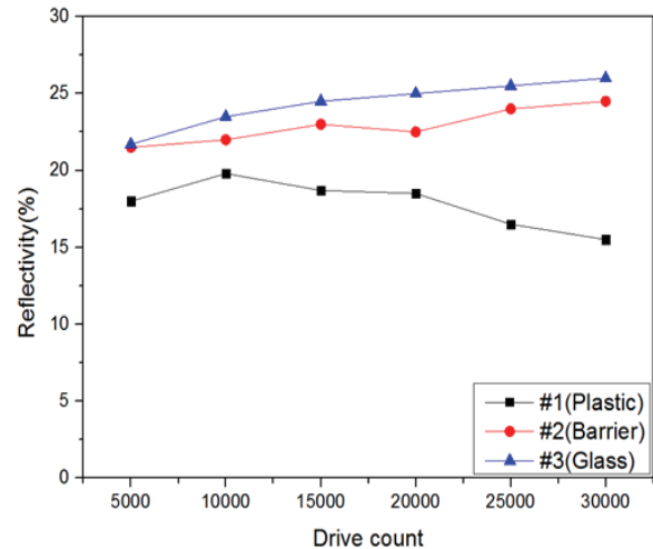
Fig. 6. Reflectivity of three sample panels according to driving count after intended degradation.
