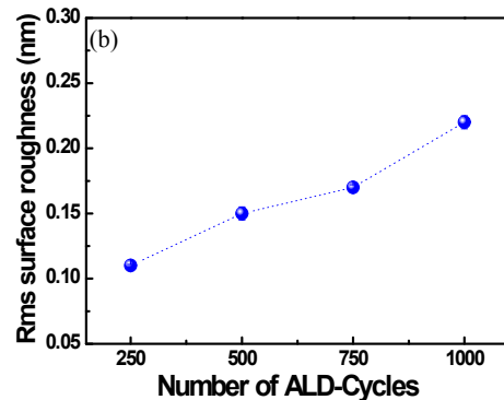
Fig. 4. (a) Surface image of TiO 2 thin films measured by AFM (1,000 ALD-cycles TiO 2 ), and (b), the change of rms surface roughness of TiO 2 films as a function of number of ALD-cycles.
