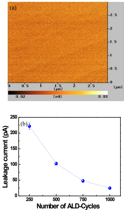
Fig. 5. (a) Surface leakage current of TiO 2 thin films measured by AFM (1,000 ALD-cycles TiO 2 ), and (b), the change of surface leakage current of TiO 2 films as a function of number of ALD-cycles.
