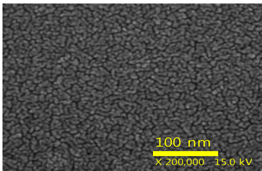
Fig. 3. FESEM surface images of TiO 2 film synthesized on silicon substrate at the condition of 1,000 cycles ALD-cycles.
