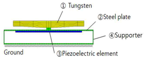
Fig. 1. Crosssectional view of the type 1 haptic actuator using piezoelectric element.
