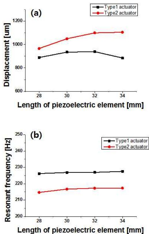
Fig. 6. Length of piezoelectric element dependence of displacement and resonant frequency of Type 1 and Type 2 actuator; (a) maximum displacement of actuator and (b) resonant frequency of actuator.
