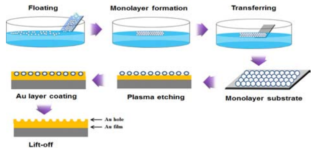
Fig. 4. Fabrication processes of polystyrene beads.
