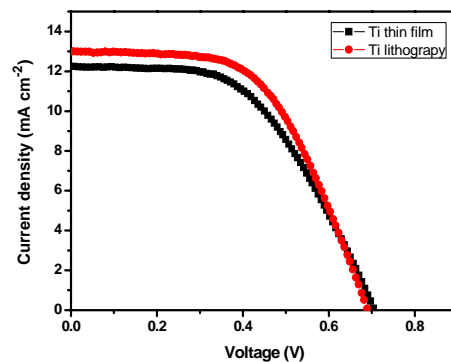
Fig. 4. Photocurrent density-voltage characteristics of DSSCs.
