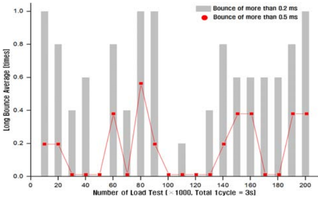
Fig. 7. Change in the average number of bounce (more than 0.2 ms, 347 V/20 A).
