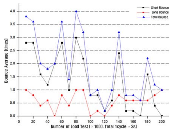
Fig. 4. Change in the average number of bounce (347 V/20 A).
