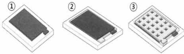
Fig. 1. Process of capacitive humidity sensor. ① lower electrode formation, ② PI pattern formation, and ③ upper electrode formation.
