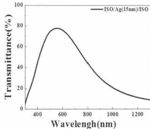
Fig. 2. Optical transmittance spectra of ISO/Ag/ISO multilayer.
