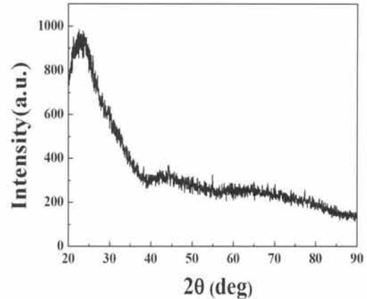
Fig. 1. The X-ray diffraction patterns of ISO single layer.
