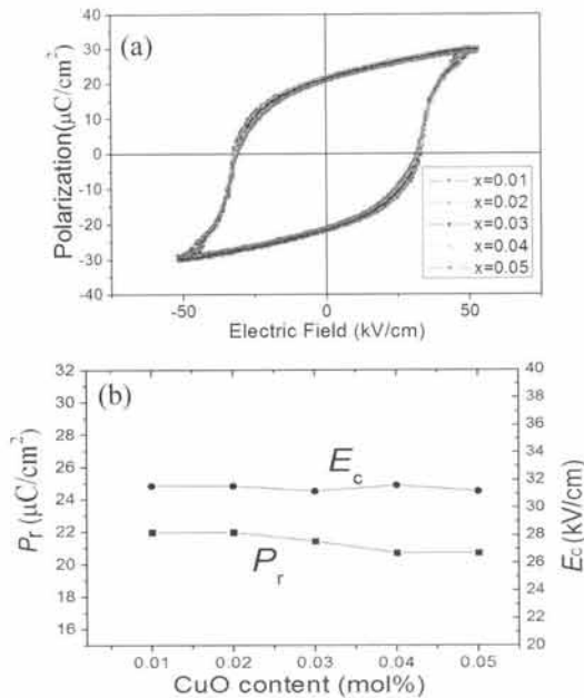
Fig. 5. Ferroelectric properties of BNKT-xCuO ceramics. (a) polarization hysteresis loops, (b) remnant polarization ( P_r ) and coercive field ( E_c ) as a function of CuO content.
