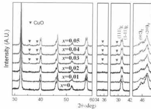
Fig. 2. X-ray diffraction patterns of BNKT- x CuO ceramics sintered at 975°C for 2 hours.
