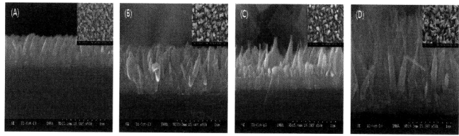
Fig. 3. FE-SEM images of the ZnO nanowires grown for 2, 4, 6, and 8 [h] by hydrothermal synthesis technique without external bias: (a) 2 [h], (b) 4 [h], (c) 6 [h], and (d) 8 [h]. [Inset is surface image of the ZnO nanowires].
