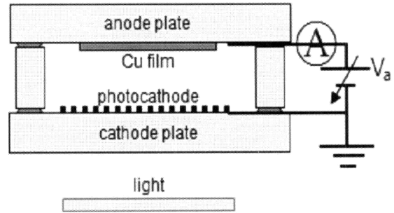
Fig. 4. Schematic diagram of photocathode device test structure.
