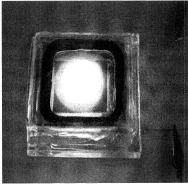
Fig. 6. Light emission of photocathode device with green phosphor at anode voltage of 10 kV.
