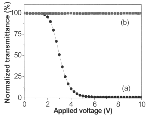
Fig. 2. V-T curve of TN cell fabricated by DFLL. (a) with 1 kHz and (b) with 50 kHz.
