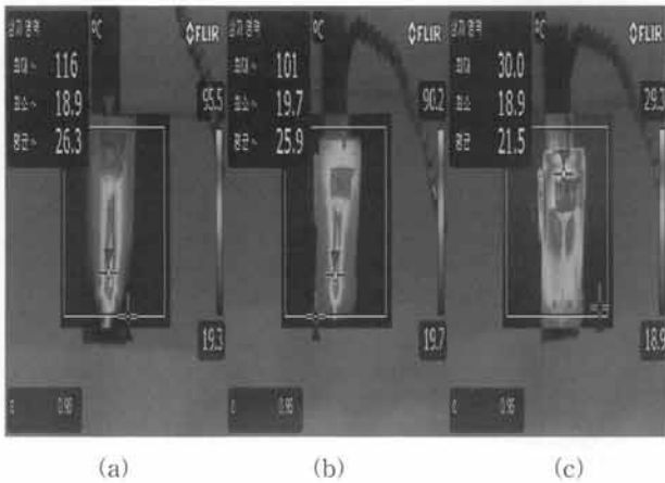
Fig. 8. Temperature properties due to thermal image in tracking degradation of silicone rubber add to reinforcing agent of (a) 30 phr, (b) 60 phr, and (c) 90 phr.
