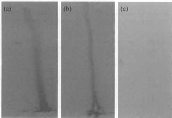
Fig. 9. Tracking degraded properties according to resistance in silicone compound with vinyl silane treated ATH, (a) 30 phr, (b) 60 phr, and (c) 90 phr.
