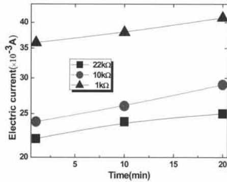
Fig. 6. Temperature properties due to I-time(min) in tracking degrade of silicone rubber add to 60 phr of reinforcing agent.
