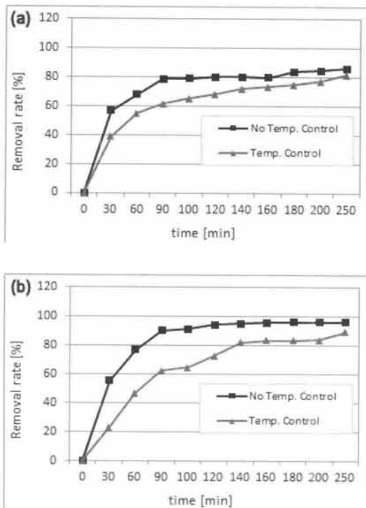
Fig. 9. Influence of TCE removal rate according to existence of temperature control: (a) 50 ppm, (b) 100 ppm.
