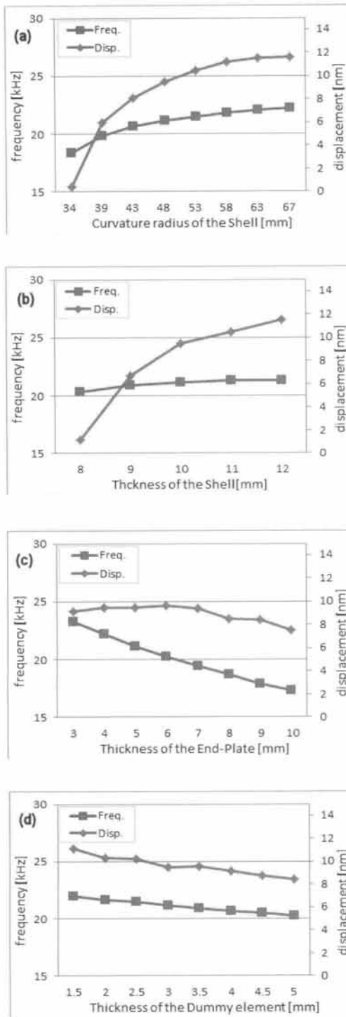
Fig. 6. Effect of the 4 design parameters on both the 1st flextensional resonant frequency and shell's horizontal displacement. (a) curvature of the shell, (b) thickness of the shell, (c) thickness of the end-plate, and (d) thickness of the Dummy element.
