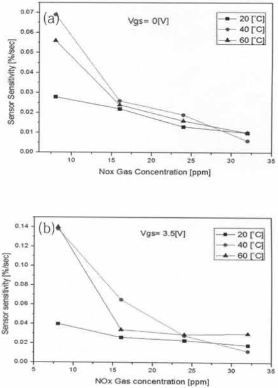
Fig. 5. Gas detection sensitivity of MWCNT gas sensor with the NOx gas. (a) V_{gs} = 0[V] , (b) V_{gs} = 3.5[V] .
