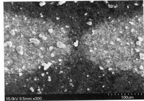
Fig. 2. The shape for the surface view of electrode.
