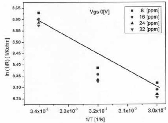
Fig. 7. The Arrhenius plot for the NOx sensing properties of MWCNT films.
