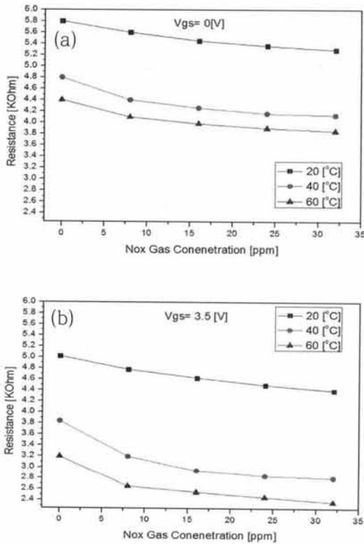
Fig. 4. Resistance change with the temperature during the adsorption of gas sensor. (a) V_{gs} = 0[V] , (b) V_{gs} = 3.5[V] .
