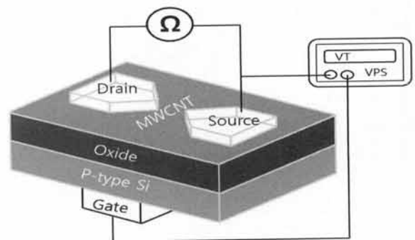
Fig. 3. Measuring system.
