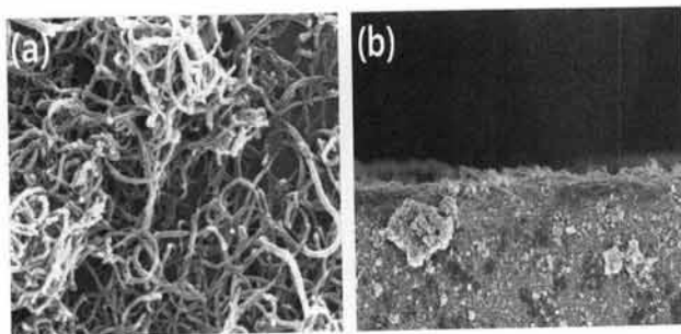
Fig. 1. The shape of the MWCNT deposited on the P-type Si-wafer. (a) MWCNT structure view, (b) cross sectional view.
