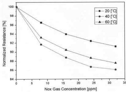
Fig. 6. The MWCNT sensor resistance change was caused by gas concentration.
