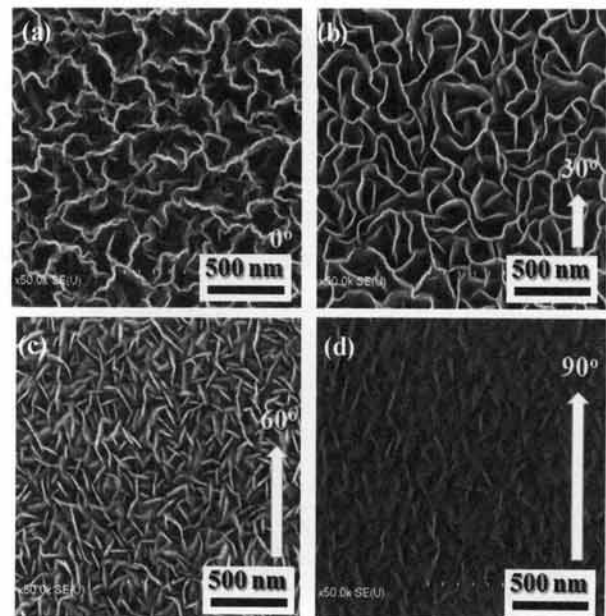
Fig. 2. Planar SEM images of CNWs according to the substrate angle, (a) 0^\circ , (b) 30^\circ , (c) 60^\circ , (d) 90^\circ .
