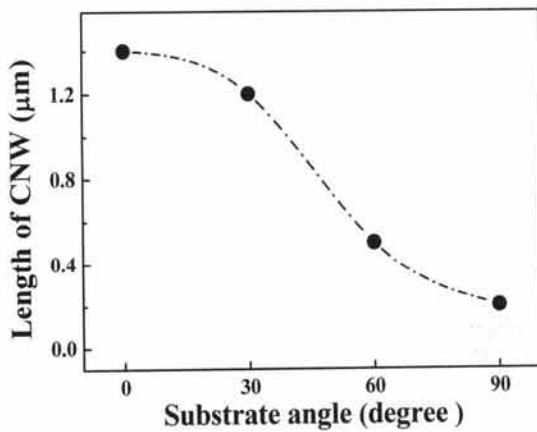
Fig. 4. Length of CNW according to the substrate angle.
