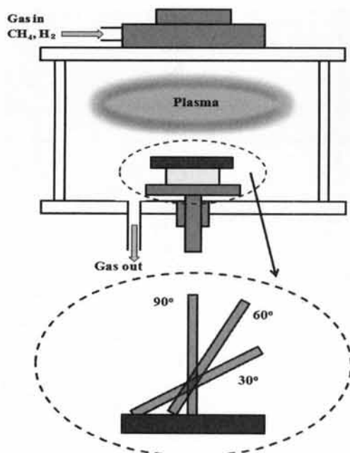
Fig. 1. Schematic of microwave PECVD and the substrate condition.
