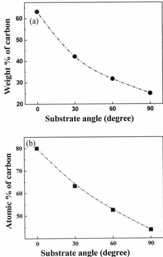
Fig. 5. EDS analysis of CNWs according to the substrate angle, (a) weight % of carbon, (b) atomic % of carbon.
