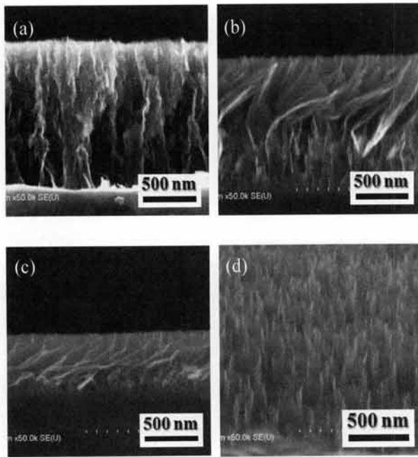
Fig. 3. Cross-sectional SEM images of CNWs according to the substrate angle, (a) 0°, (b) 30°, (c) 60°, (d) 90°.
