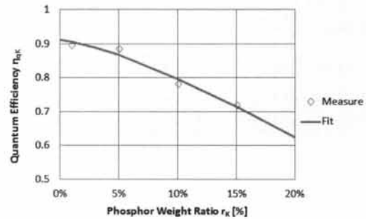
Fig. 11. Measured and model parameter fit quantum efficient \eta_{qK} .
