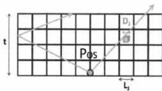
Fig. 4. Optical path in flat mold LED.
