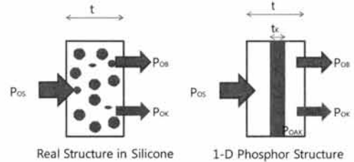
Fig. 2. 1-D modeling of 1 phosphor in silicone.
