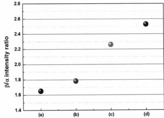
Fig. 3. Relative intensity ratios of \beta_{110}/\alpha_{020} from the above XRD diffraction patterns.
