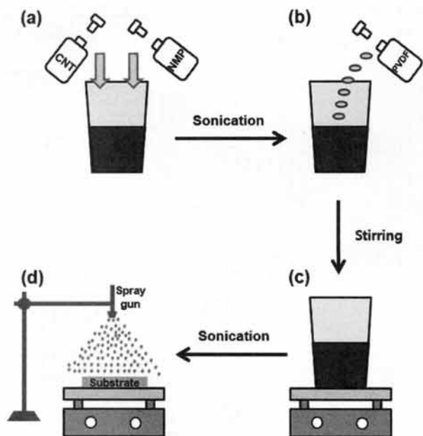
Fig. 1. Process flow of the CNT/PVDF film fabrication; (a) CNT/NMP solution preparation, (b) CNT/PVDF composite solution preparation, (c) dispersion of CNT/PVDF composite solution, and (d) CNT/PVDF film fabrication by spray coating method.
