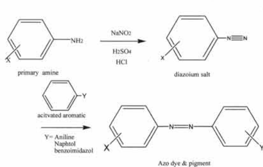
Scheme 1. Diazonium salt formation reaction of primary aromatic amine and \text{HNO}_2 and azo coupling reaction.
