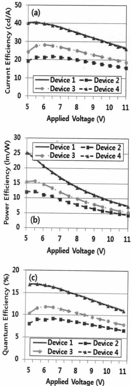
Fig. 3. Efficiency characteristics of OLED with position change of co-doping white emitting layer and blue emitting layer (a) current efficiency vs applied voltage, (b) power efficiency vs applied voltage, (c) quantum efficiency vs applied voltage.
