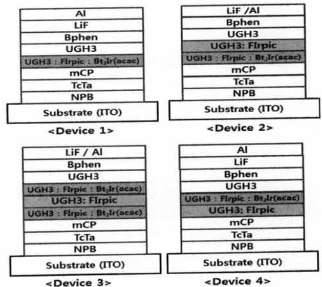
Fig. 1. Device structure of OLED with position change of co-doping white emitting layer and blue emitting layer.
