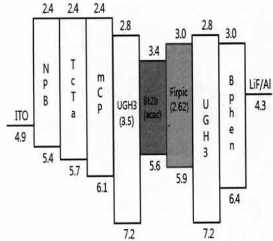
Fig. 5. Energy level diagram of fabricated phosphorescent OLED.
