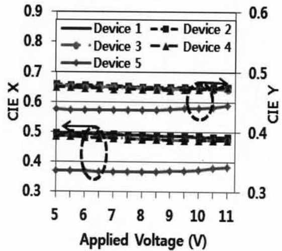
Fig. 8. Commission internationale de l'Éclairage (CIE) coordinates of OLED with position change of co-doping white emitting layer and blue emitting layer.
