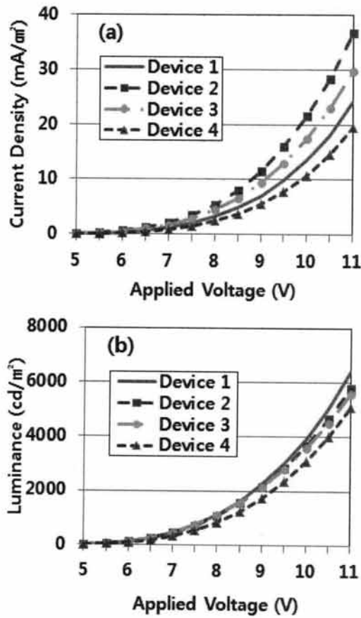
Fig. 2. Current and luminance characteristics of OLED with position change of co-doping white emitting layer and blue emitting layer. (a) current density vs applied voltage, (b) luminance vs applied voltage.
