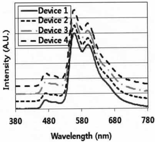
Fig. 4. Electroluminescence spectra of OLED with position change of co-doping white emitting layer and blue emitting layer.
