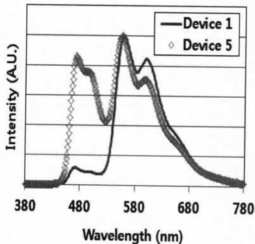
Fig. 7. The electroluminescence spectra of OLED with co-doping and OLED inserted with UGH3 : FIrpc of 5 nm thickness.
