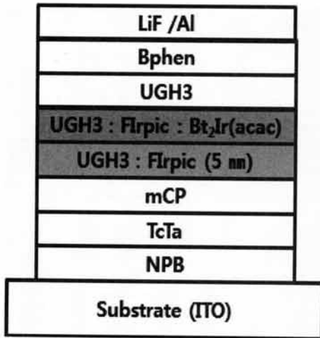
Fig. 6. Device structure of OLED with UGH3 : FIrpc of 5 nm thickness.
