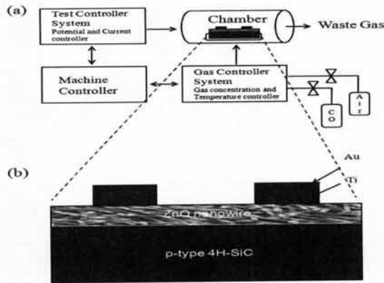
Fig. 1. Schematic diagram of (a) gas sensor measurement system, (b) ZnO nanowire/SiC gas sensor.
