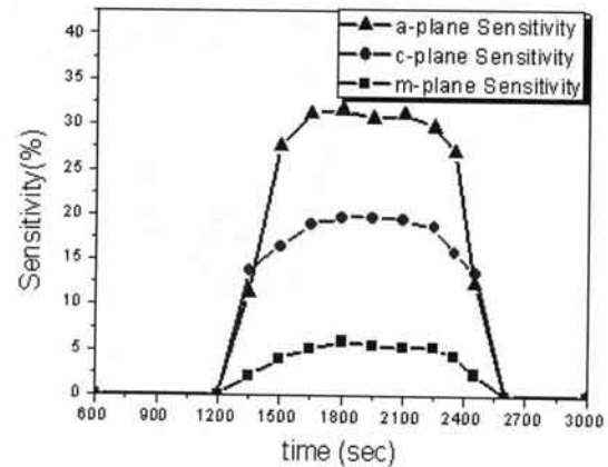
Fig. 5. CO gas sensitivity of ZnO nanowires based on the a-, c- and m-plane 4H-SiC.
