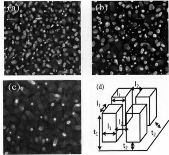
Fig. 2. Top view FE-SEM images of ZnO nanowires grown on (a) a-plane oriented, (b) c-plane-oriented, (c) m-plane oriented 4H-SiC substrates and Geometric model of nanowire structure showing parameters to estimate effective thickness.
