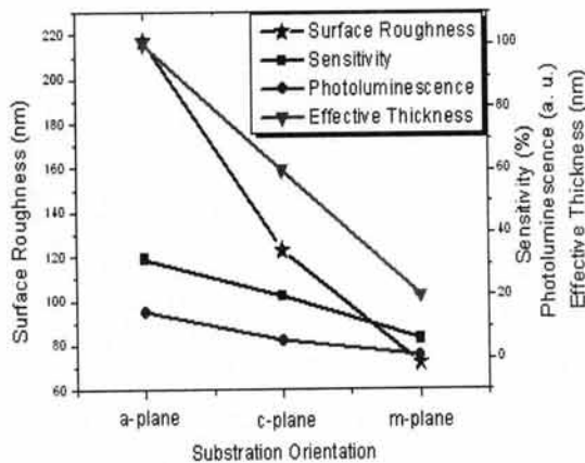
Fig. 6. Surface roughness dependent to sensitivity, photoluminescence and effective thickness.
