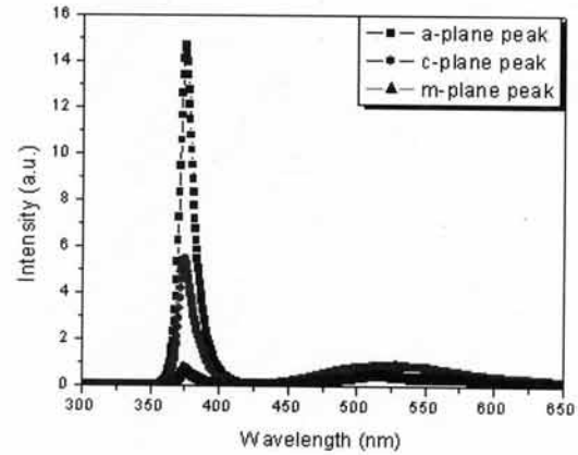
Fig. 4. Photoluminescence spectrum of ZnO nanowires grown on a-, c-, and m-plane oriented 4H-SiC substrates.
