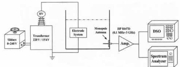
Fig. 7. Configuration of the experimental setup.
