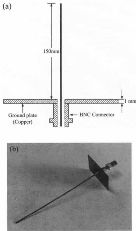
Fig. 5. Prototype monopole antenna. (a) schematic diagram, (b) photograph.
