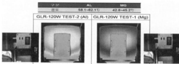
Fig. 3. Heat dissipation shape and actual temperature measurements.
