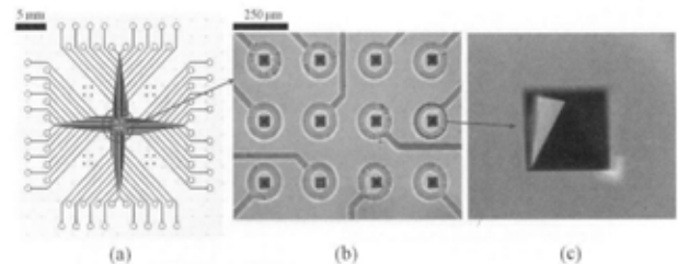
Fig. 2. A micrograph of a single PPL probe consisting of a circular membrane and pyramidal tip (a) design layout of an active PPL array, (b) close-up micrograph of a PPL array section, (c) a pyramidal tip.
