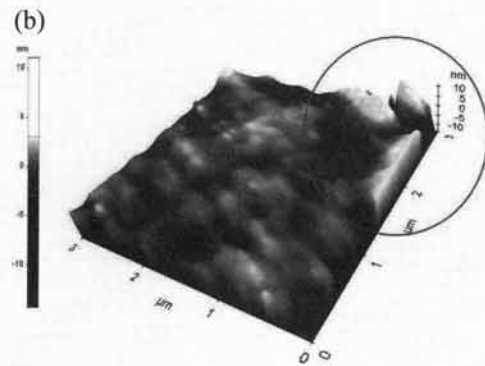
Fig. 5. AFM images on solution processed MSL HfO 2 layers with oblique ion beam exposure. (a) MSL HfO 2 layer, (b) ML HfO 2 layer.
