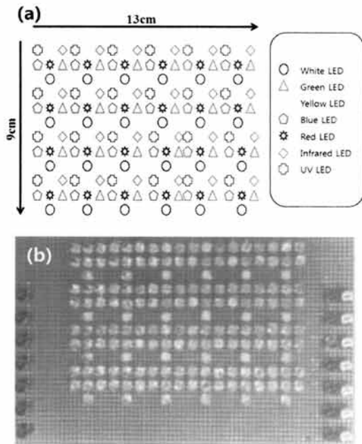
Fig. 2. (a) Schematic illustration of LEDs arrangement, (b) photograph of LED solar simulator.
