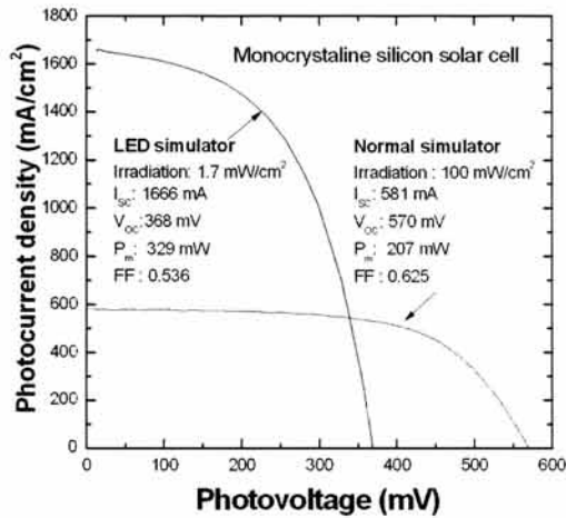
Fig. 4. I-V characteristic of mono-crystalline solar cells using LED solar simulator and Xenon lamp solar simulator.
