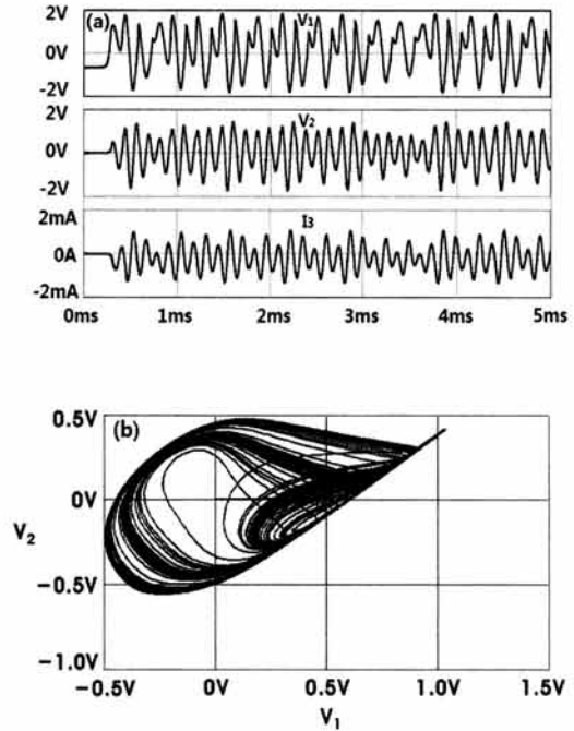
Fig. 4. Chaotic dynamics according to the variation of the Chua's diode (M 1 , M 2 W/L= 60 \mu\text{m}/2 \mu\text{m} ). (a) time waveform (V 1 , V 2 , I 3 ), (b) phase plane (V 1 , V 2 ).
