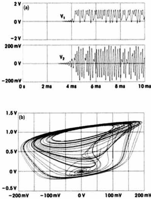
Fig. 9. Phase plane of V1 and V2 in condition - 0°C. (a) time waveform (V1, V2), (b) phase plane (V1, V2).
