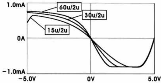
Fig. 3. I-V curves of the transconductor based Chua's diode according to the variation of MOS sizes.
