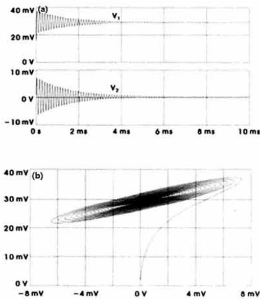
Fig. 13. Phase plane of V1 and V2 in condition 200°C. (a) time waveform (V1, V2), (b) phase plane (V1, V2).
