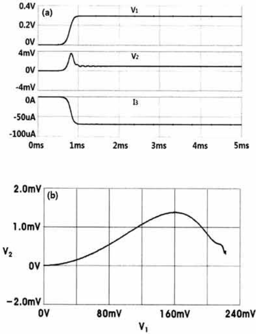
Fig. 6. Chaotic dynamics according to the variation of the Chua's diode ( M_1, M_2 W/L= 15 \mu\text{m}/2 \mu\text{m} ). (a) time waveform ( V_1, V_2, I_3 ), (b) phase plane ( V_1, V_2 ).
