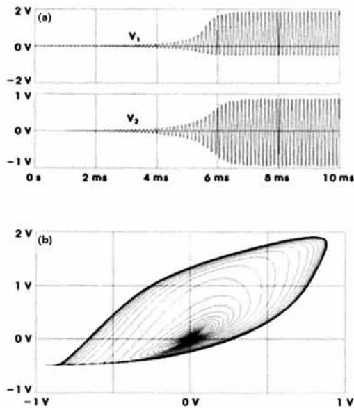
Fig. 12. Phase plane of V1 and V2 in condition 100°C. (a) time waveform (V1, V2), (b) phase plane (V1, V2).
