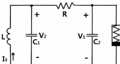
Fig. 1. Transconductor based Chua's chaotic circuit.
