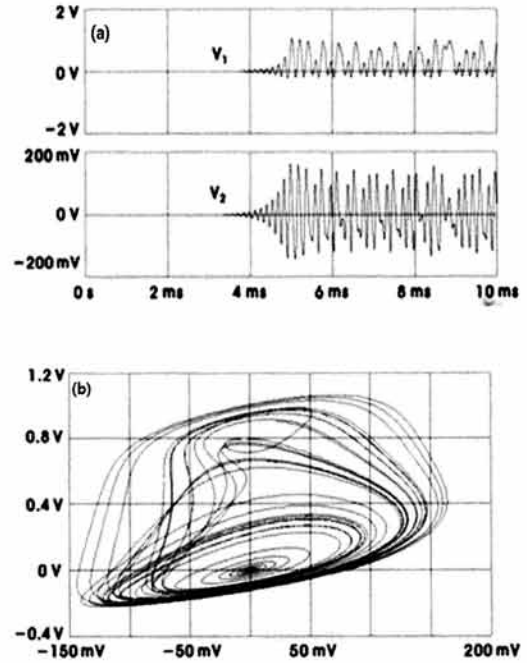
Fig. 10. Phase plane of V1 and V2 in condition 27°C. (a) time waveform (V1, V2), (b) phase plane (V1, V2).
