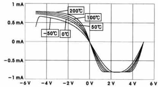
Fig. 7. I-V curves of the transconductor based Chua's diode according to the variation of the temperature dependence.
