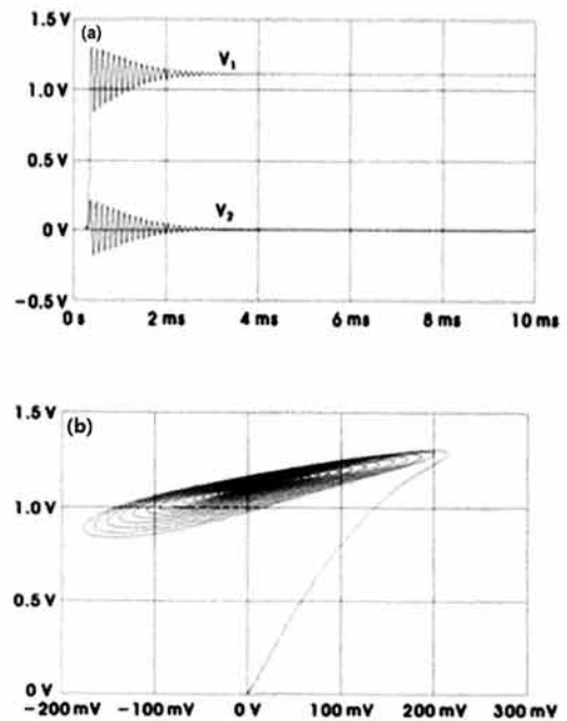
Fig. 8. Phase plane of V_1 and V_2 in condition -50^\circ\text{C} (a) time waveform ( V_1, V_2 ), (b) phase plane ( V_1, V_2 ).
