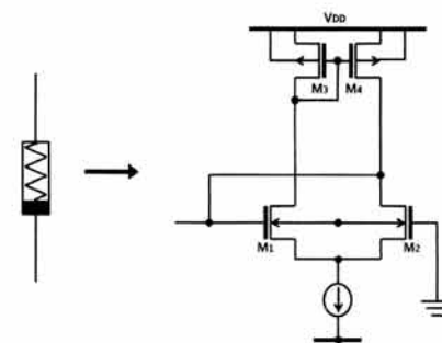
Fig. 2. Schematic of the transconductor based Chua's diode.
