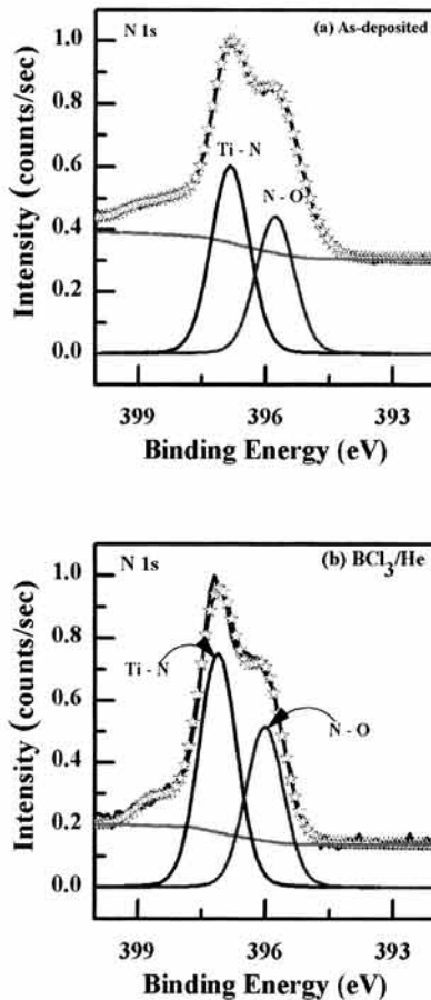
Fig. 5. X-ray photoelectron spectroscopy narrow scan spectra of the etched TiN thin film of N 1s. (a) As-deposited, (b) BCl 3 /He plasma.
