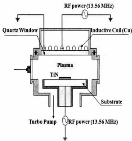
Fig. 1. Schematic of inductively coupled plasma system.
