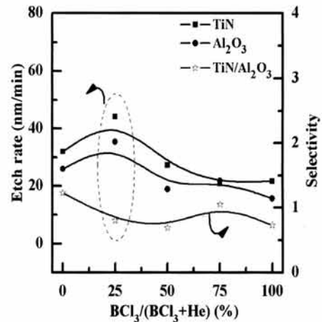
Fig. 2. The etch rate of the TiN tin films and selectivity of TiN to Al 2 O 3 as a function of the gas mixing ratio.
