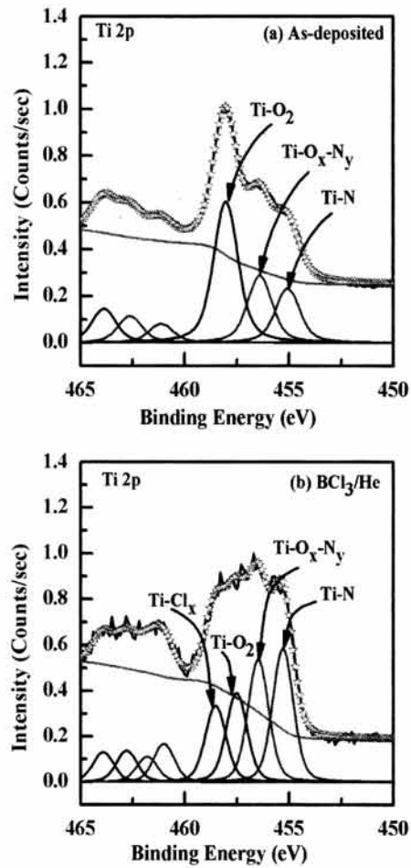
Fig. 4. X-ray photoelectron spectroscopy narrow scan spectra of the etched TiN thin film of Ti 2p. (a) As-deposited, (b) BCl 3 /He plasma.
