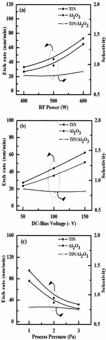
Fig. 3. The etch rate of the TiN tin films and selectivity of TiN to Al 2 O 3 as a function of (a) RF power, (b) DC-Bias voltage, (c) process pressure.
