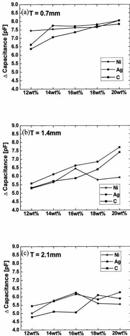
Fig. 7. According to the depth variation, materials and mixture fraction in capacitance change. (a) depth(thickness) 0.7 mm, (b) depth(thickness) 1.4 mm, (c) depth(thickness) 2.1 mm.
