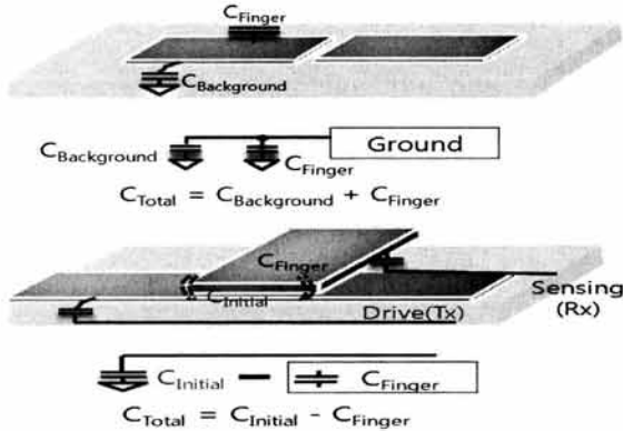
Fig. 1. Capacitive type touch panel driving method. Self type(top), mutual type(bottom).
