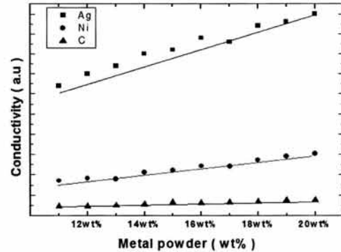
Fig. 5. PDMS + metal powder theoretical conductivity of composite material.
