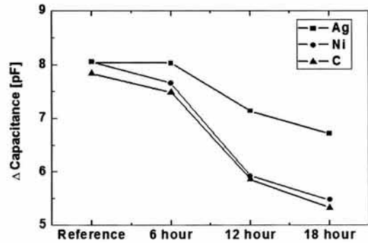
Fig. 6. According to the milling time variation in capacitance change.
