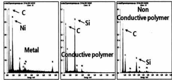
Fig. 2. Component analysis of stylus pen.
