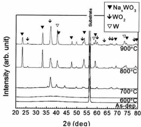
Fig. 10. X-ray diffraction patterns of the thin films of \text{Na}_{0.75}\text{WO}_3 composition annealed in vacuum at various temperatures.
