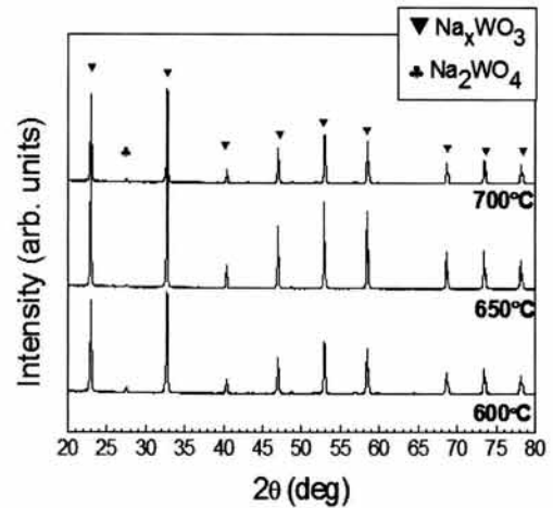
Fig. 2. X-ray diffraction patterns of the powders of \text{NaWO}_3 composition calcined at various temperatures for 10 hours in 5% \text{H}_2/\text{Ar} atmosphere.
