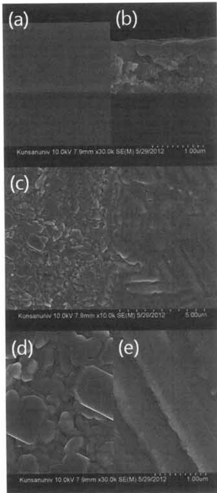
Fig. 12. Cross-sectional FE-SEM images of the thin films of \text{Na}_{0.75}\text{WO}_3 composition: (a) as-deposited and (b) annealed at 800^\circ\text{C} in vacuum. (c) Plane-view image of the film annealed at 800^\circ\text{C} in vacuum. Magnified images of (d) the left side and (e) the right side of (c).
