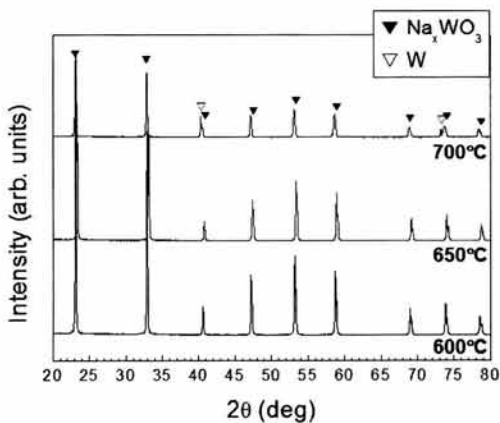
Fig. 4. X-ray diffraction patterns of the powders of \text{Na}_{0.75}\text{WO}_3 composition calcined at various temperatures for 10 hours in 5\% \text{H}_2/\text{Ar} atmosphere.
