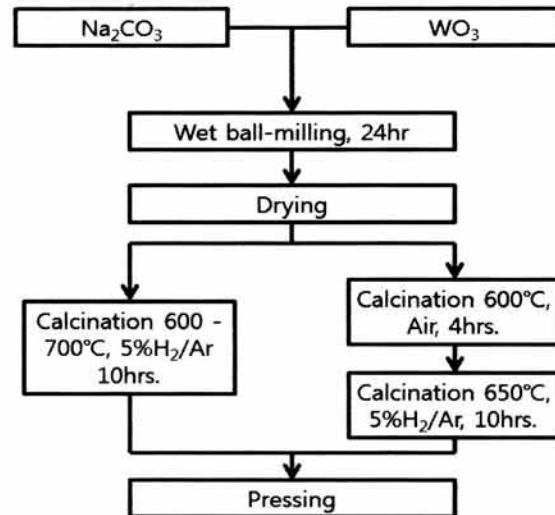
Fig. 1. Flow chart for the preparation of \text{Na}_x\text{WO}_3 powder targets.
