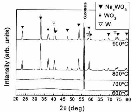
Fig. 11. X-ray diffraction patterns of the thin films of \text{Na}_{0.75}\text{WO}_3 composition annealed in Ar atmosphere at various temperatures.
