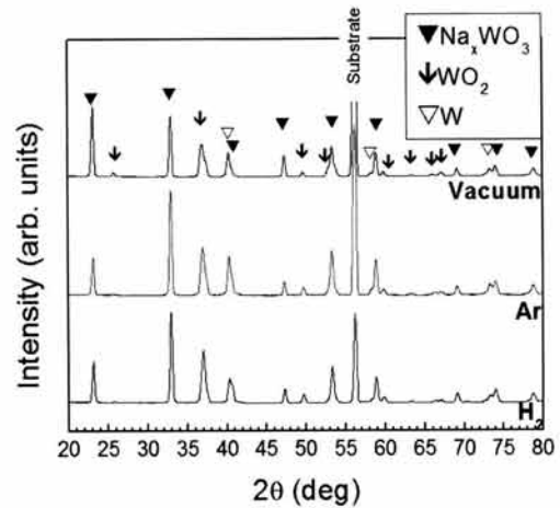
Fig. 9. X-ray diffraction patterns of the thin films of \text{Na}_{0.75}\text{WO}_3 composition annealed by RTP at 800^\circ\text{C} in various atmospheres.
