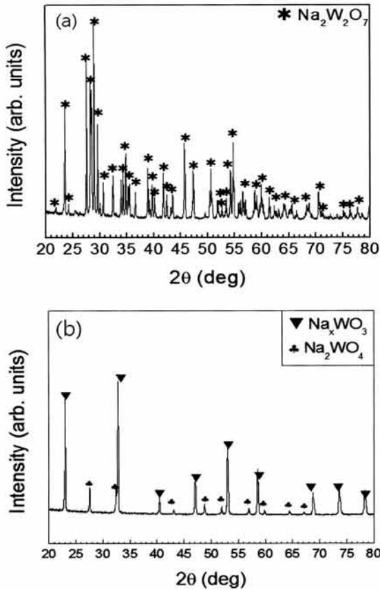
Fig. 3. X-ray diffraction patterns of the powders of \text{NaWO}_3 composition (a) calcined at 600^\circ\text{C} in air for 4 hours (first step) and (b) calcined at 600^\circ\text{C} in air for 4 hours followed by an annealing at 650^\circ\text{C} in 5\% \text{H}_2/\text{Ar} atmosphere for 10 hours (first step + second step).
