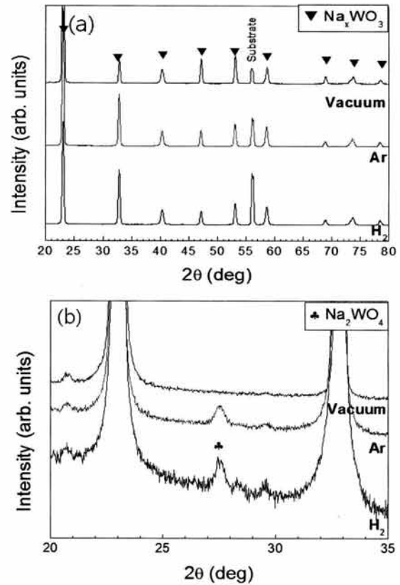
Fig. 6. (a) X-ray diffraction patterns of the thin films of NaWO 3 composition annealed by RTP at 800℃ in various atmospheres. (b) magnified patterns of (a) between 20° and 35°.
