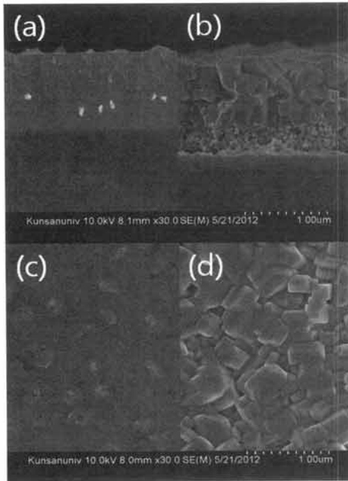
Fig. 8. Cross-sectional FE-SEM images of the thin films of \text{Na}_x\text{WO}_3 composition: (a) as-deposited and (b) annealed at 800^\circ\text{C} in vacuum. Plane-view images: (c) as-deposited and (d) annealed at 800^\circ\text{C} in vacuum.
