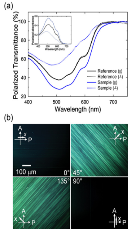
Fig. 2. (a) Polarized transmission and absorption (inset) spectra of the reference and sample PV layers for incident light polarized parallel ( \parallel ) and perpendicular ( \perp ) to the rubbing direction of the PV layers, (b) polarizing microscopic textures of the sample PV layer at four angles of rotation of the layers. The white arrows indicate the rubbing ( x -) direction and the orientation of the crossed polarizers is shown by the crossed arrows (A, P).
