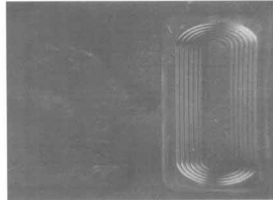
Fig. 3. Photographs of the fabricated sensor with Lincoln face in penny.
