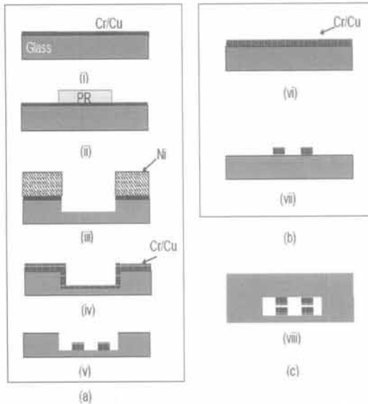
Fig. 2. Fabrication sequence for the sensor. (a) bottom, (b) top, and (c) bonding.
