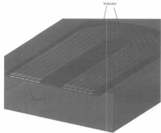
Fig. 1. Schematic of micromachined wireless pressure.
