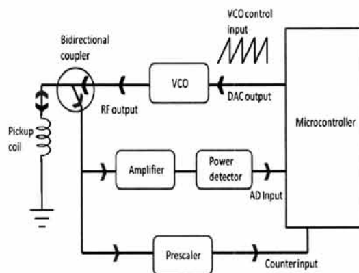
Fig. 5. Schematic of pressure readout circuit.
