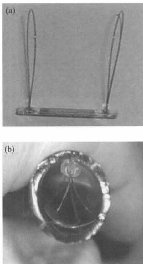
Fig. 4. (a) sensor with nitinol basket and (b) sensor in artery simulating tubing.
